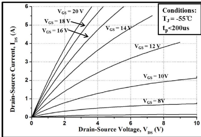
Figure 1. Output Characteristics T_J = -55^{\circ}C
