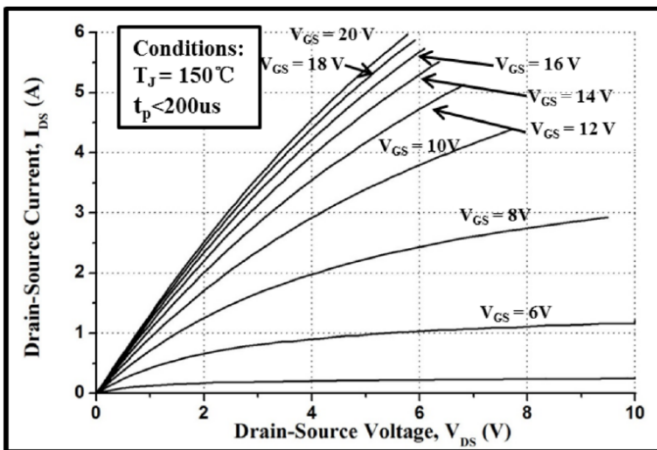
Figure 3. Output Characteristics T_J = 150^{\circ}C
