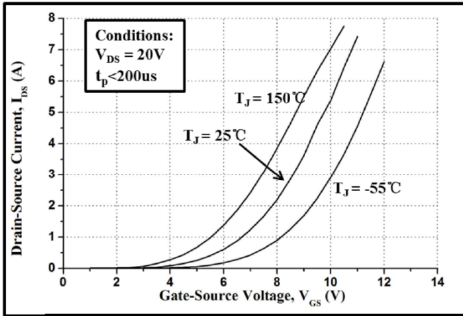
Figure 5. Transfer Characteristic for Various Junction Temperatures
