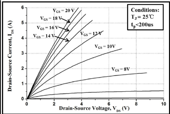
Figure 2. Output Characteristics T_J = 25^{\circ}C
